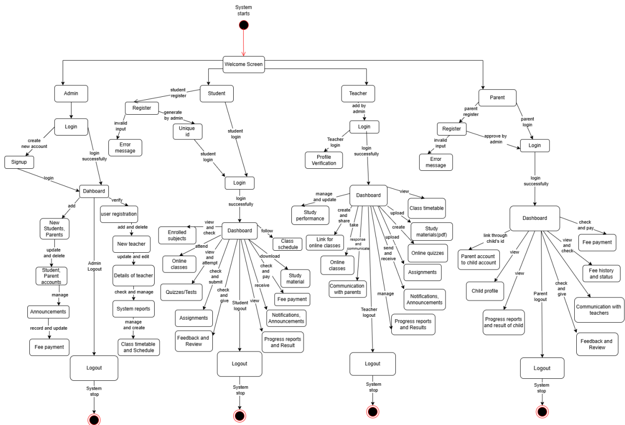
Figure 9: State Diagram
