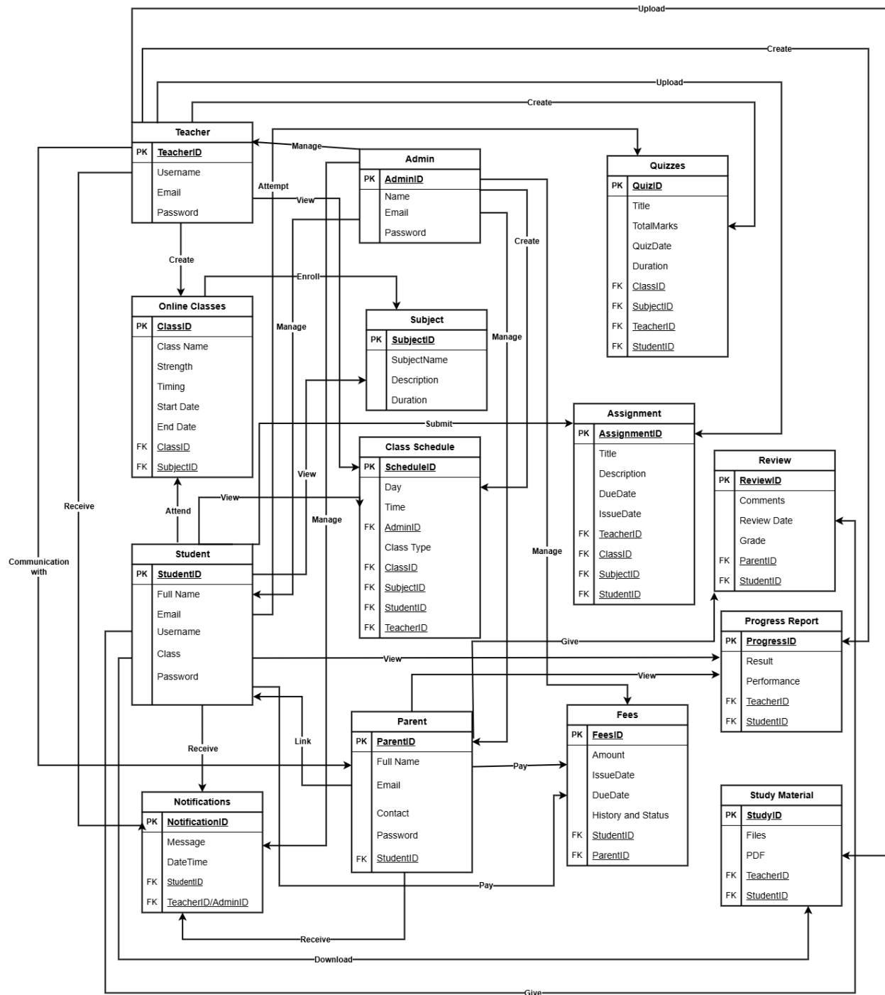
Figure 12: ERD Schema
