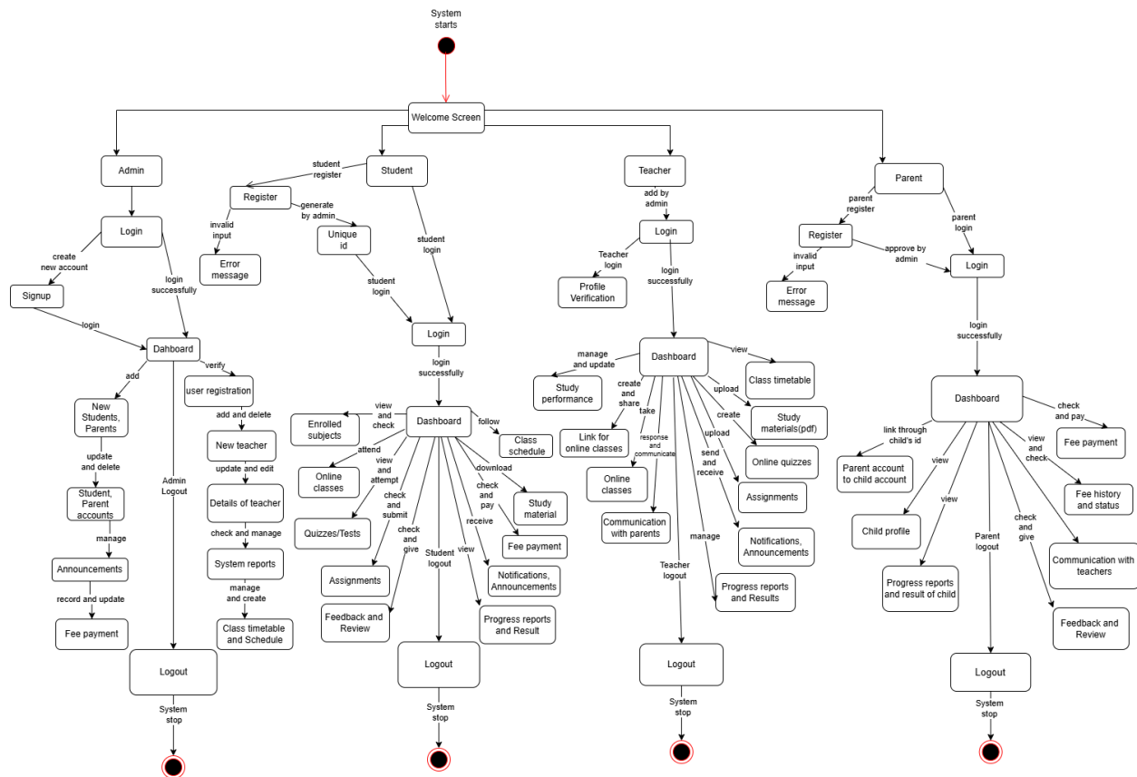
Figure 21: State Diagram
