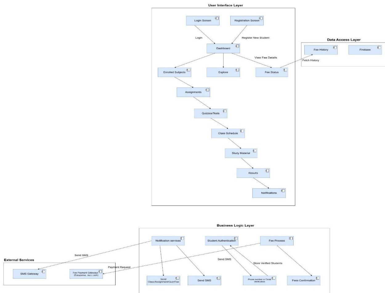
Figure 10: Architecture Diagram
